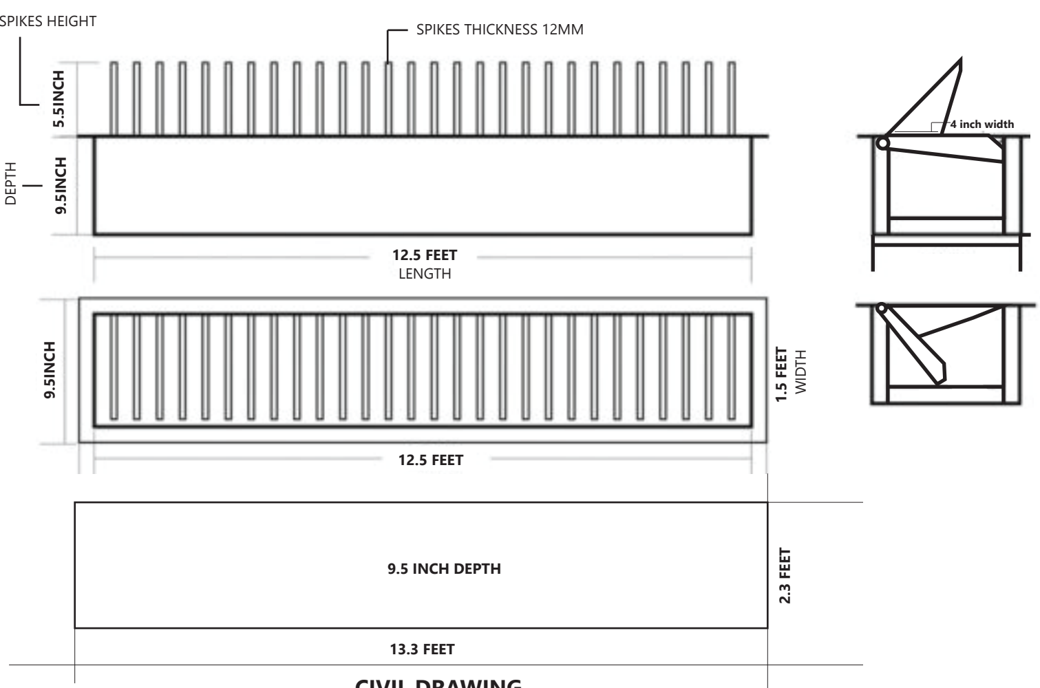
CIVIL DRAWING
